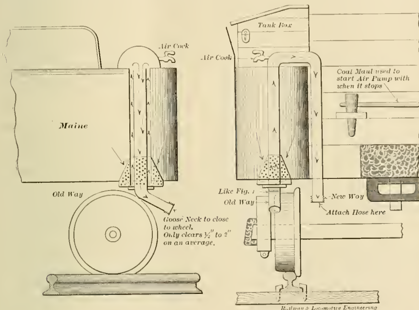
TANK STRAINER FOR INJECTORS.
